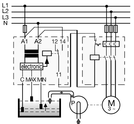
CM-ENS.2x, CM-ENS.31 Liquid level control - fill - selected function "↑" (UP)
