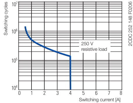
Contact lifetime
