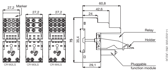
CR-M2LS - CR-M3LS - CR-M4LS - screw connection
