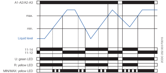
Fill: CM-ENS.2x
